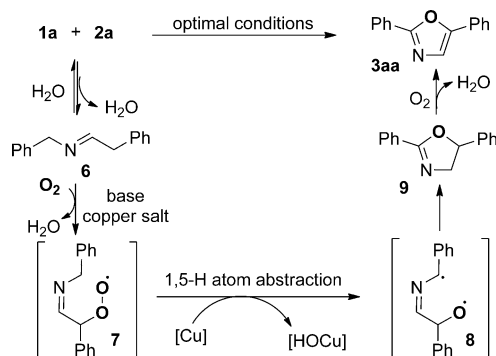
Scheme 3. Possible reaction pathway for dioxygen activation and oxazole formation.
